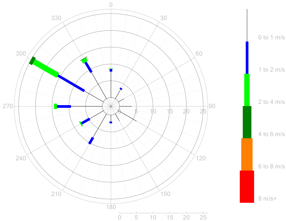
Figure 9:WCX Bridgewater Park - Wind Rose of June 2023
