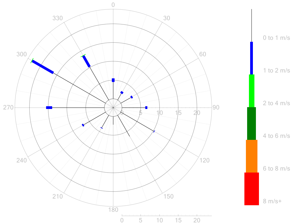
Figure 8:WCX Manning Street - Wind Rose of June 2023
