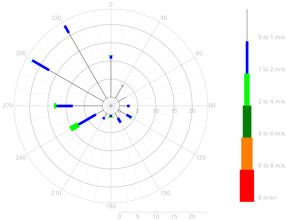
Figure 6: WCX Quirk Street - Wind Rose of June 2023
