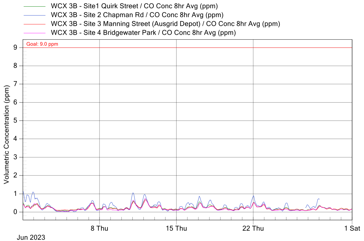
Figure 2: WCX 3B Project Air Monitoring Stations - CO 8-Hour Rolling Graph for June 2023
