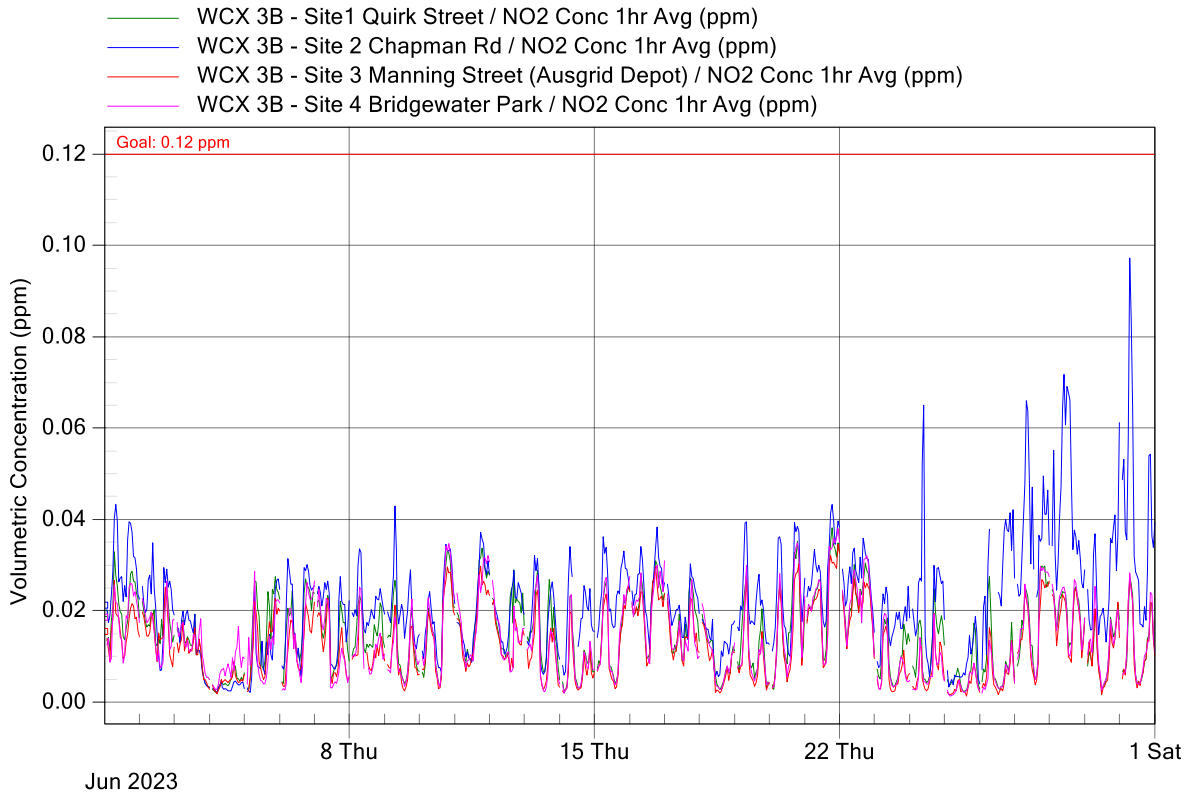
Figure 3: WCX 3B Project Air Monitoring Stations - NO 2 1-Hour Averages Graph for June 2023
