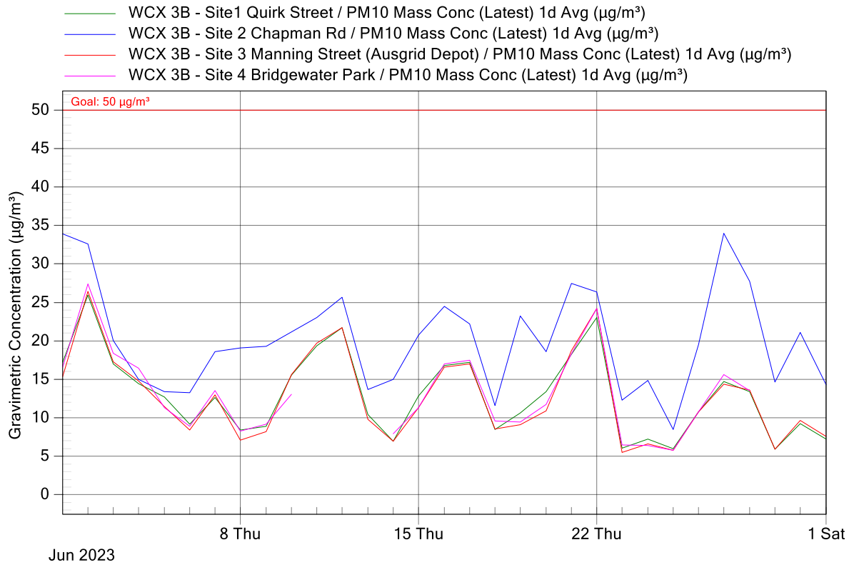
Figure 4: WCX 3B Project Air Monitoring Stations - PM 10 24-Hour Averages Graph for June 2023
