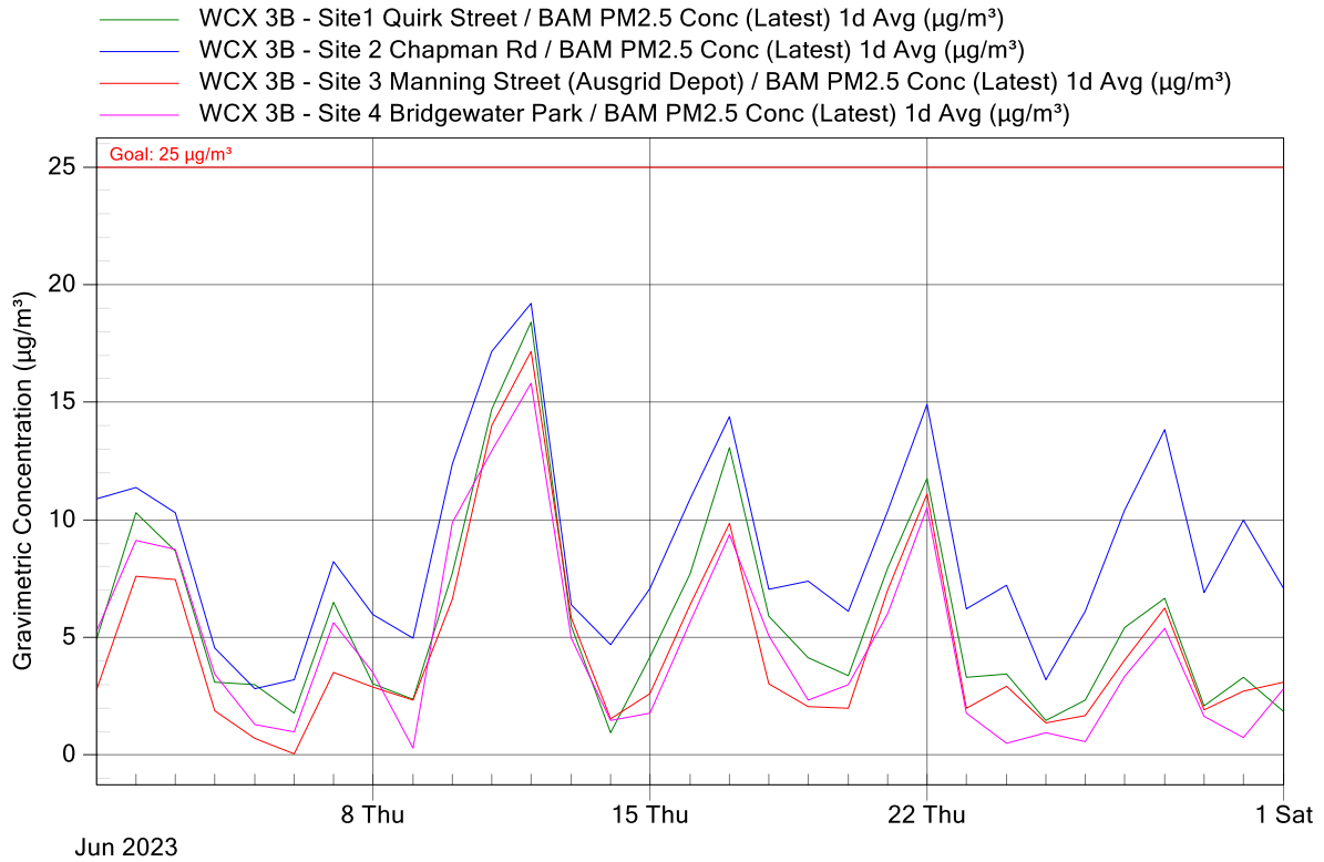
Figure 5: WCX 3B Project Air Monitoring Stations - PM 2.5 24-Hour Averages Graph for June 2023
