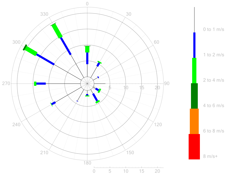
Figure 7:WCX Chapman Road - Wind Rose of June 2023
